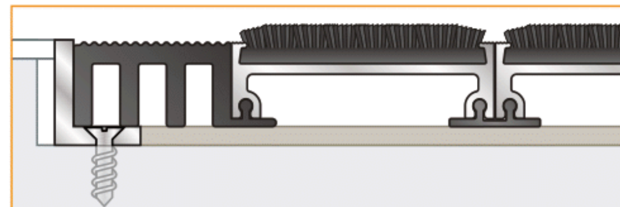
Rigid PVC finishing strips (to be cut) supplied on the ends of the mat and used for adjustment in the matwell.
